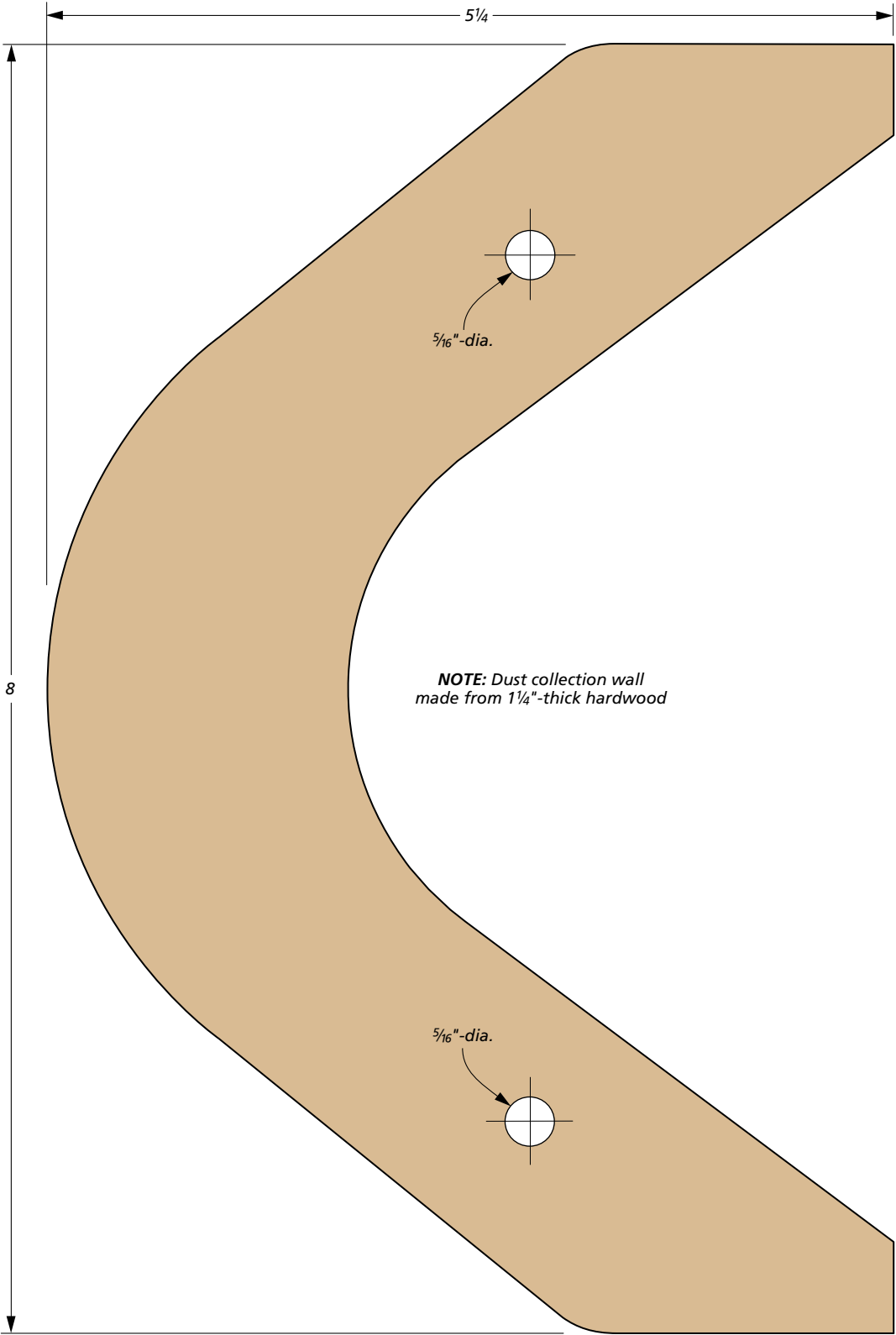
PATTERN DUST COLLECTION WALL (Full-size)
