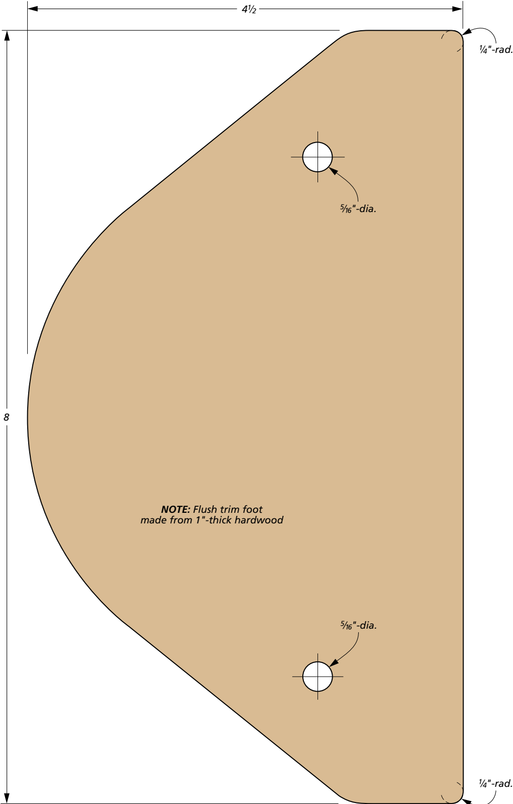
PATTERN FLUSH-TRIM FOOT (Full-size)
